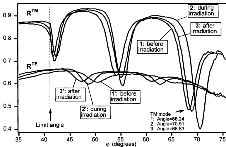
FIGURE 4 TM and TE reflectivity versus the incidence angle for P1 film.
